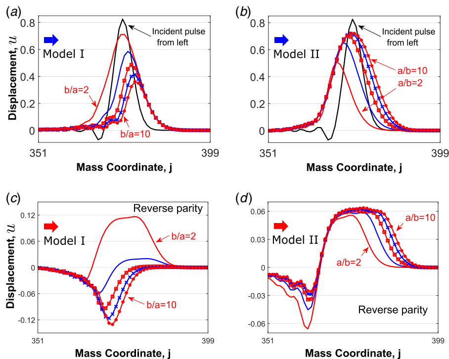
Fig. 6 Transmitted amplitudes for the two models in Fig. 5: (a) and (c) model I on the left and (b) and (d) model II on the right. The curve indicated in (a) and (b) is the incident CT pulse; other curves represent the transmitted waves. Transmitted results for incidence from the left for model I are in (a) and from the right in (c), in both cases for b/a = 2, 4, 6, 8, 10 , demonstrating very significant non-reciprocal transmission; similar phenomena are evident in (b), the results of incidence from the left, and (d), incidence from the right, which consider a/b = 2, 4, 6, 8, 10 for model II.
