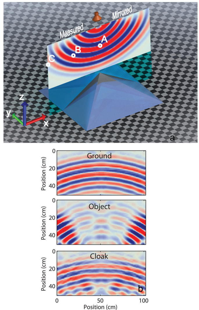
Figure 6. (a) The setup for the 3D carpet cloak of Figure 5. (b) Measured reflected pressure fields for three cases: ground only, object, object+cloak. Reprinted from (Zigoneanu et al., 2014) with permission. (Movie version https://www.youtube.com/watch?v=k13L8u2tACY )
