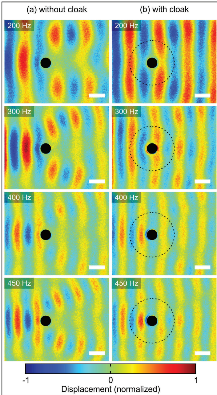
Figure 7. Cloaking of flexural waves. The black cloaked region of diameter 3 cm is clamped, the dashed lines depict the outer boundary of the cloak. Reprinted from (Stenger et al., 2012) with permission. This movie shows experimental results at 200 Hz. (To view movie please visit http://wp.me/p4zu0b-MY )
