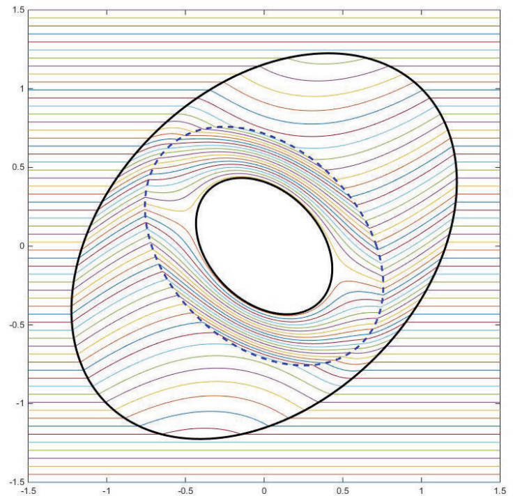
Figure 4. Ray paths through a non-radially symmetric cloak. The solid curves are the inner and outer surface of the cloak.
