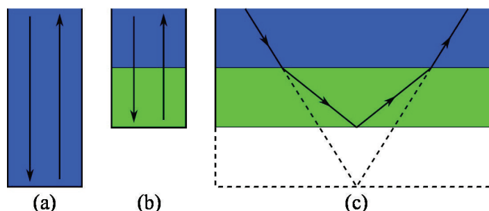
Figure 1. Some space is made available in (b) by shrinking a region of (a) into the transformed green material. As explained in the text, the original and transformed ray paths in (c) imply that the transformed medium must display acoustic anisotropy. The wave speed in the horizontal direction is unchanged while the vertical speed is lower than the original.
