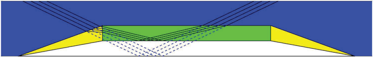
Figure 2. A carpet cloak. The white region is freed up by squashing the entire white+green+yellow region into the green and yellow segments. The green region is a one dimensional compression, as in Figure 1. The transformation in the yellow region depends on both the vertical and horizontal coordinates, resulting in a compression and an extension in orthogonal directions not aligned with the coordinates axes (Craster and Guenneau, 2013, Ch. 7).
