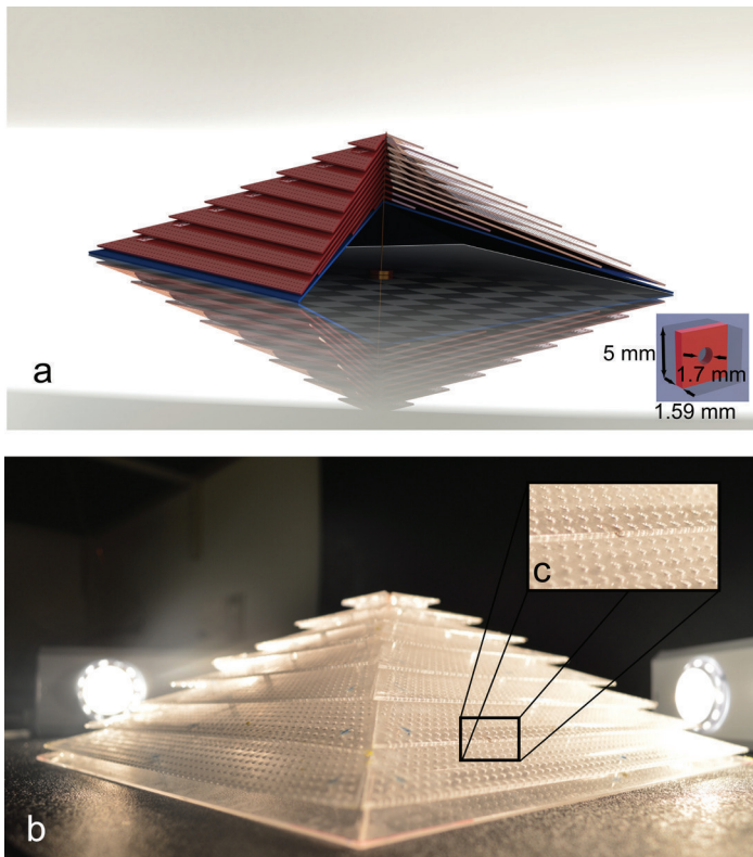
Figure 5. The pyramidal acoustic carpet cloak of Zigoneanu et al. (2014). Reprinted with permission.
