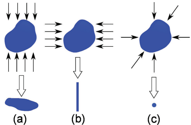
Figure 3. (a) The cloaked region is flattened by a one dimensional-like mapping. (b) The cloaked region has the scattering cross-section of a thin cylinder. (c) A fully 3D transformation; the cloaked region scatters like a point.
