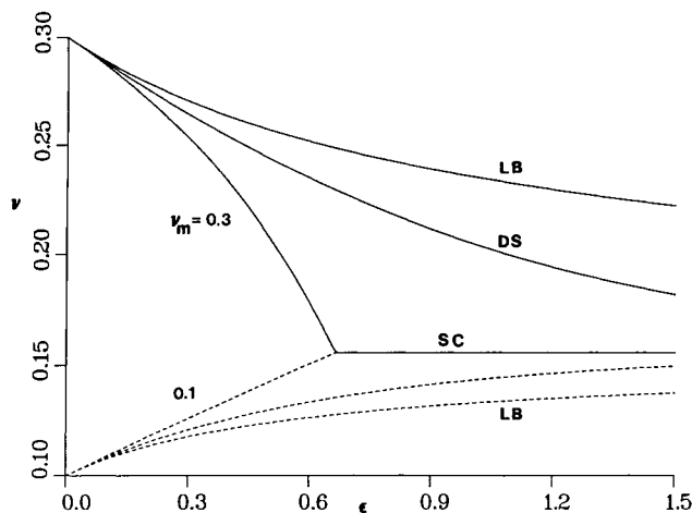
Fig. 3. The Poisson's ratio corresponding to Figs 1 and 2.
