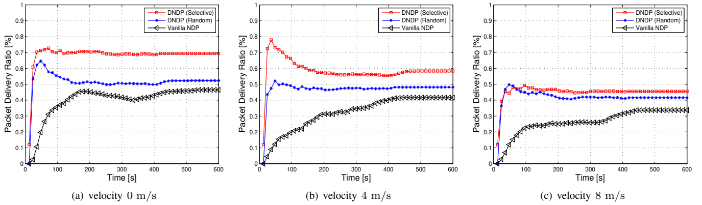
Fig. 3. Cumulative Packet Delivery Ratio vs. Time for various velocities, 16 nodes deployment.
