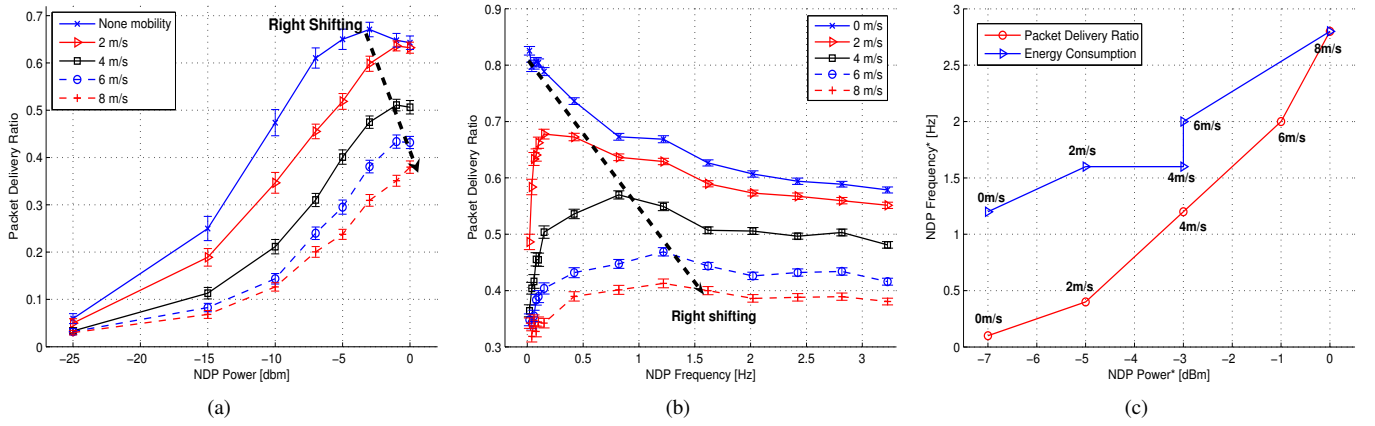
Fig. 2. (a) Packet delivery ratio vs. NDP power with mobility at NDP frequency, 1 Hz for 36 nodes; (b) Packet delivery ratio vs. NDP frequency with 0dBm NDP power for various velocities; (c) Optimal NDP frequency vs. optimal power.
